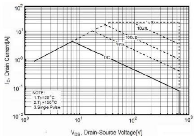
Maximum Safe Operating Area For JS60R540FU
