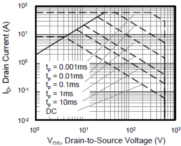
Maximum Safe Operating Area For JS60R190FU
