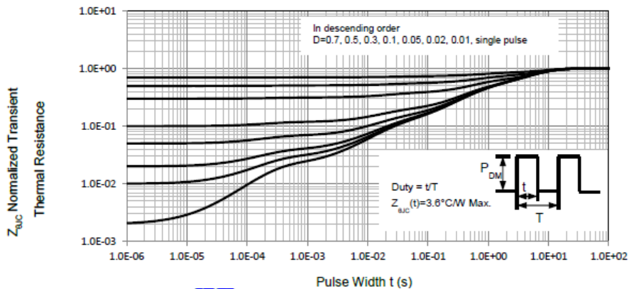
Transient Thermal Response Curve For JS60R190FU
