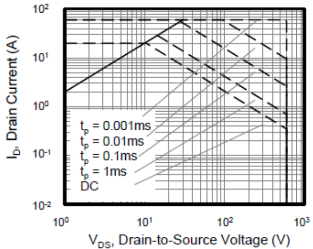
Maximum Safe Operating Area For JS60R190WU
