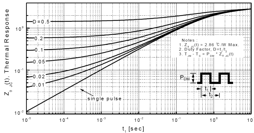
Transient Thermal Response Curve For JCS9N50F (TO-220MF)
