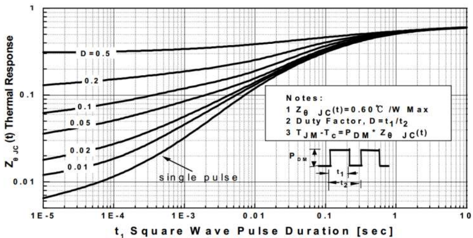
Transient Thermal Response Curve For JCS90N10I(TO-220C)
