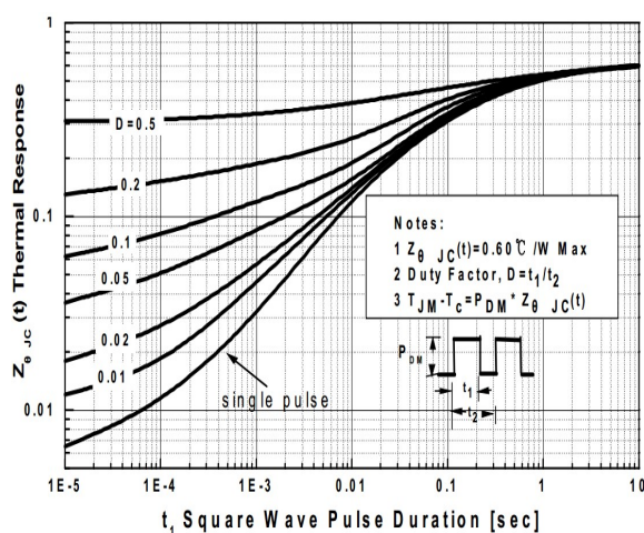
Transient Thermal Response Curve For JCS90N10I(TO-220C)
