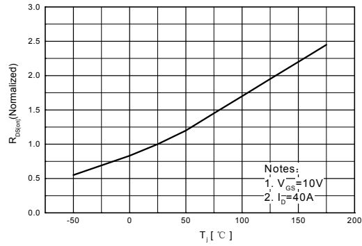
On-Resistance Variation vs. Temperature
