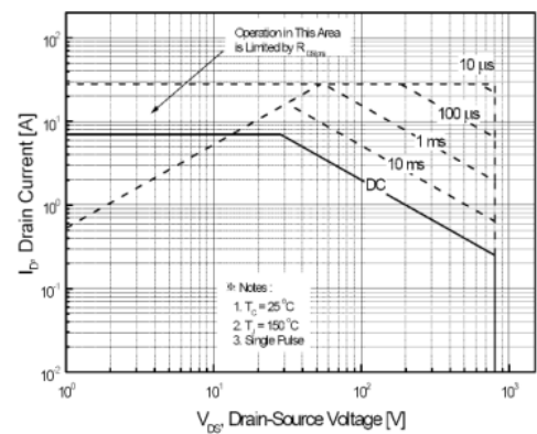
Maximum Safe Operating Area for JCS7N80FH
