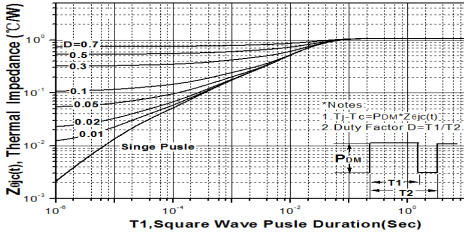
Transient Thermal Response Curve For JCS7N70VE/RE
