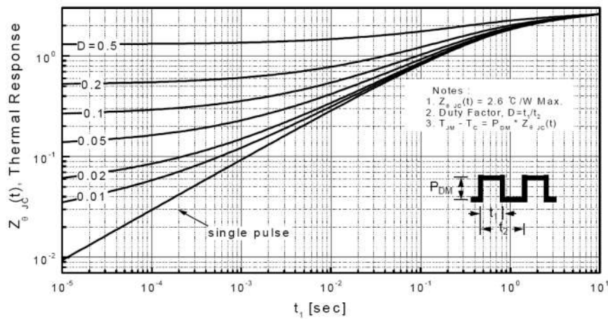
Transient Thermal Response Curve For JCS7N65F
