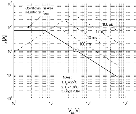
Maximum Safe Operating Area For JCS7N65F
