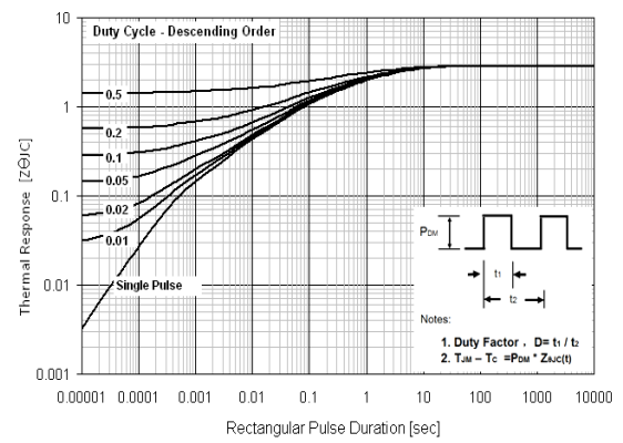
Transient Thermal Response Curve For JCS7N65FEI(TO-220MF-K1/K2/K4)
