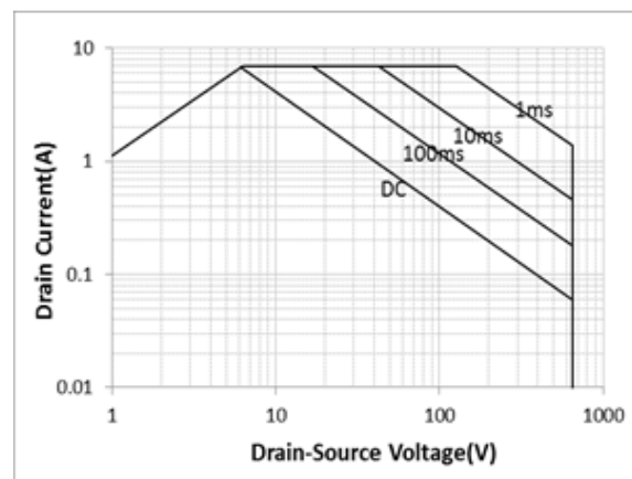
Maximum Safe Operating Area For JCS7N65FEI(TO-220MF-K1/K2/K4)
