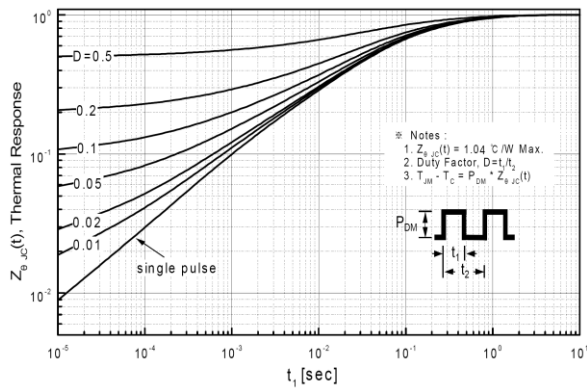
Transient Thermal Response Curve For JCS7N65CEI/SEI/BEI/REI/VEI
