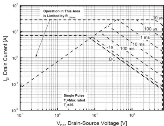
Maximum Safe Operating Area For JCS7N65CEI/SEI/BEI/REI/VEI
