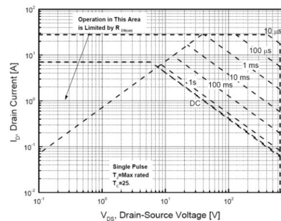
Maximum Safe Operating Area For JCS7N65CE/SE/BE/RE/VE
