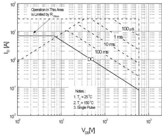
Maximum Safe Operating Area For JCS7N60F
