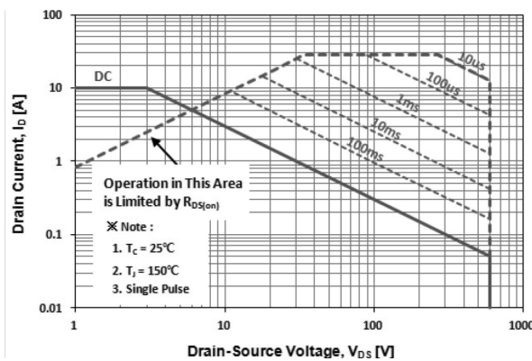
Maximum Safe Operating Area For JCS7HN60FC(TO-220MF-K1/K2)
