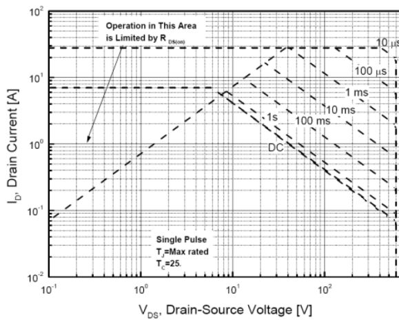
Maximum Safe Operating Area For JCS7HN60FC(TO-220MF-K1/K2)
