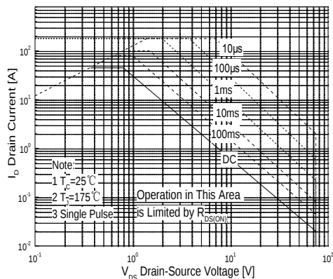
Maximum Safe Operating Area For JCS75N75FF
