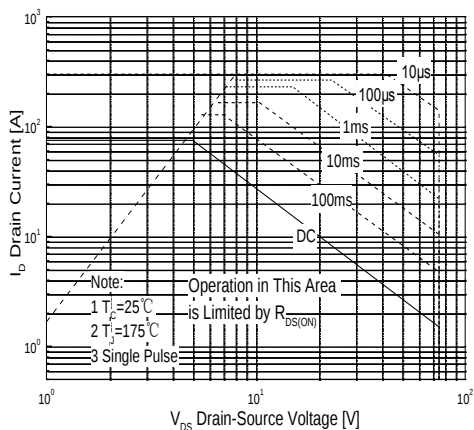
Maximum Safe Operating Area For JCS75N75CF/SF
