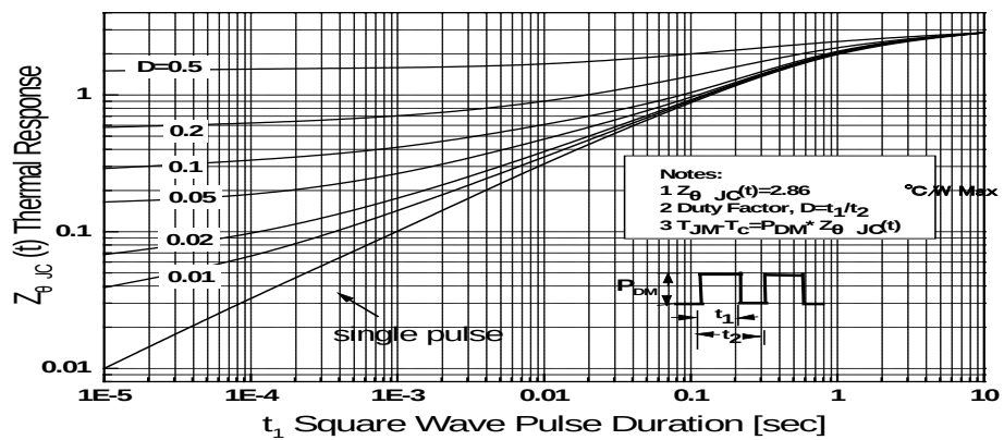
Transient Thermal Response Curve For JCS740FC
