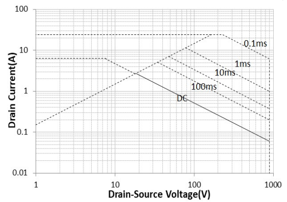
Maximum Safe Operating Area JCS6N90FH
