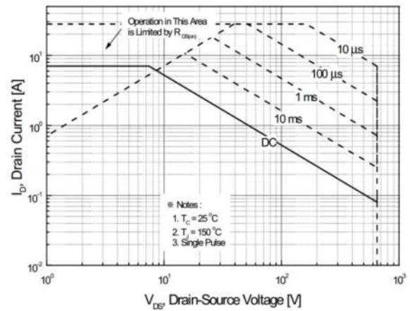
Maximum Safe Operating Area For JCS6HN65FC(TO-220MF)
