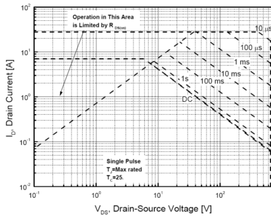
Maximum Safe Operating Area For JCS6HN65FC(TO-220MF-K2)
