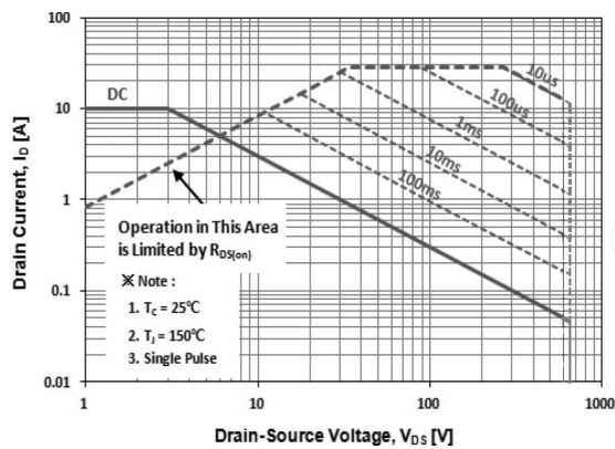
Maximum Safe Operating Area For JCS6HN65FC(TO-220MF-K2)
