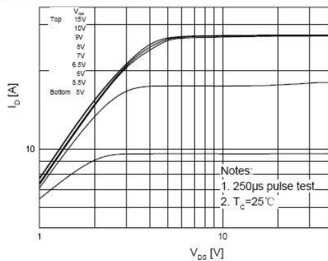
On-Region Characteristics
