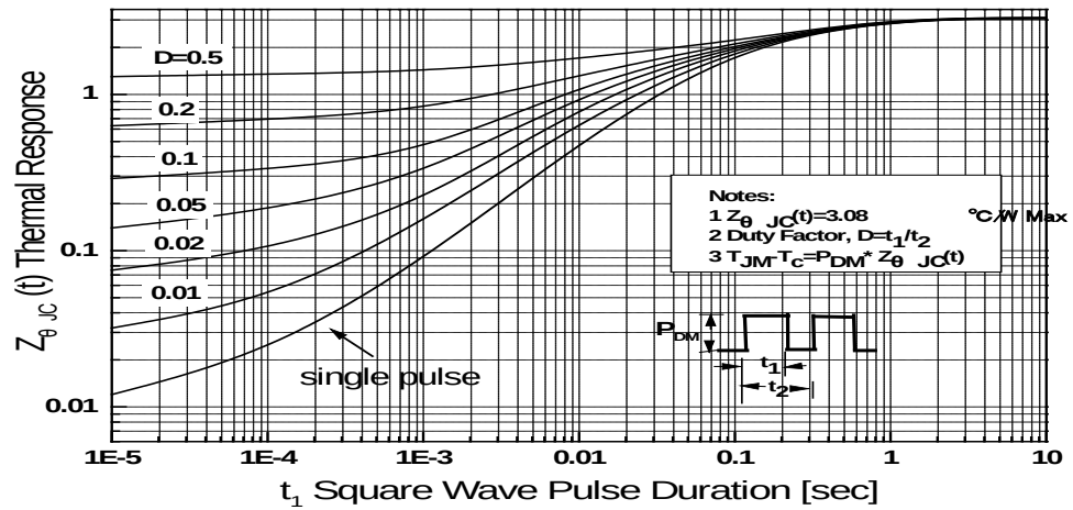
Transient Thermal Response Curve For JCS5N50FTR
