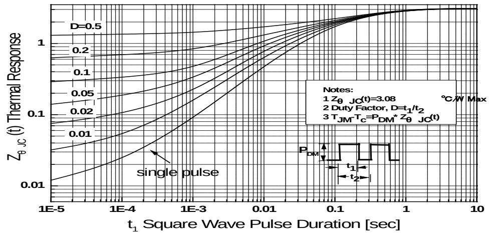
Transient Thermal Response Curve For JCS5N50FC
