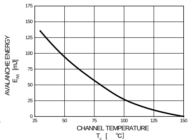
Avalanche Energy vs. Channel Temperature
