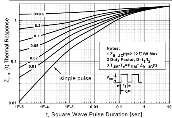
Transient Thermal Response Curve JCS50N06FH
