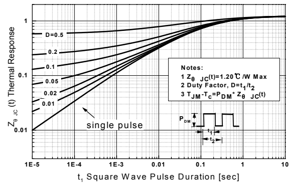
Transient Thermal Response Curve JCS50N06FH
