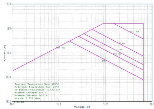
Maximum Safe Operating Area For JCS4N65REI/VEI
