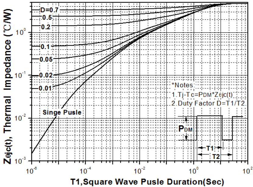
Transient Thermal Response Curve For JCS4N65FEI(TO-220MF-K1/K2/K4)
