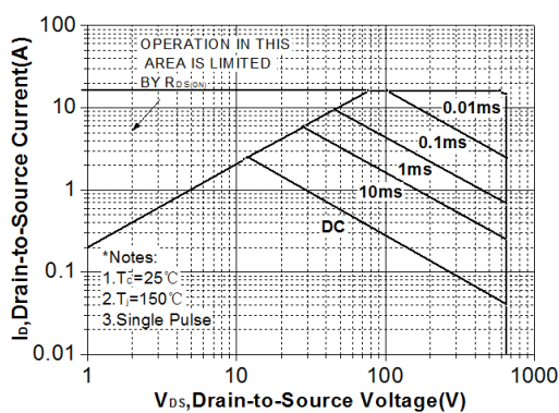
Maximum Safe Operating Area For JCS4N65FEI(TO-220MF-K1/K2/K4)
