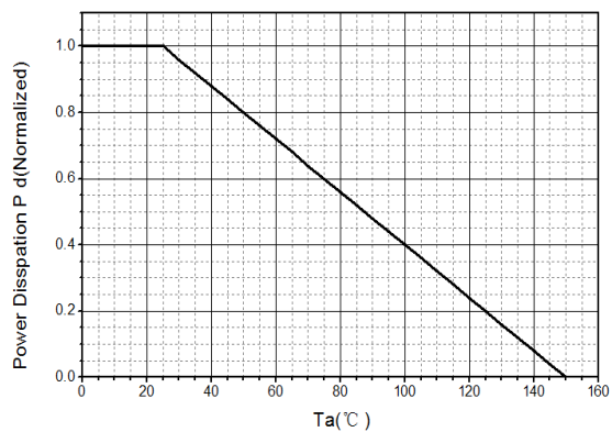
Power Dissipation vs Ta
