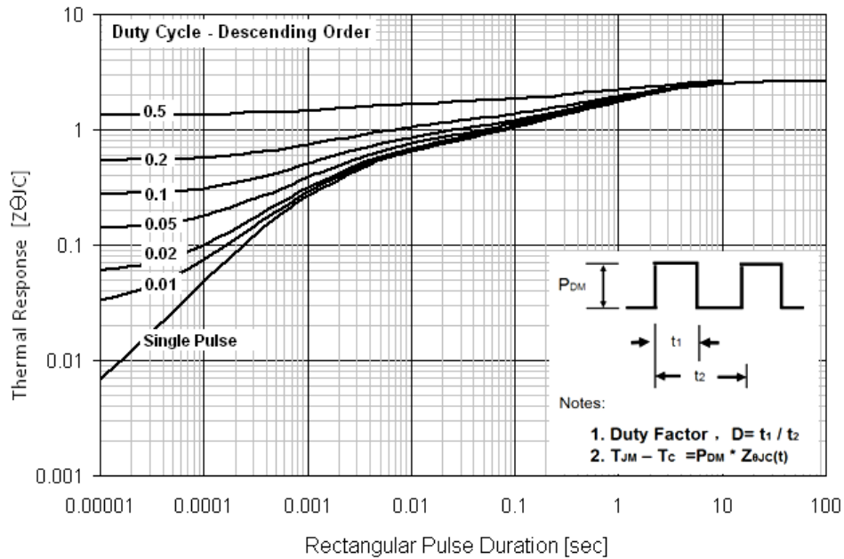
Transient Thermal Response Curve For JCS4N65FEI(TO-220MF-K2)
