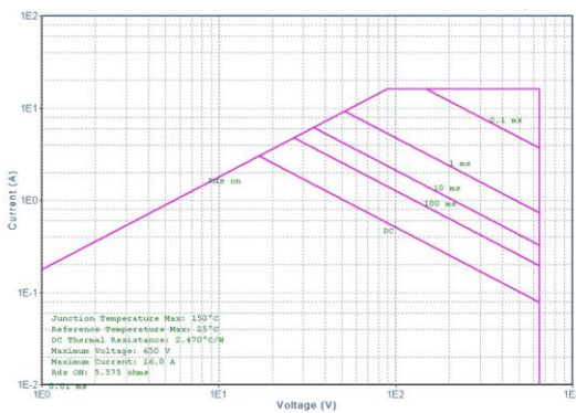
Maximum Safe Operating Area For JCS4N65FEI(TO-220MF-K2)
