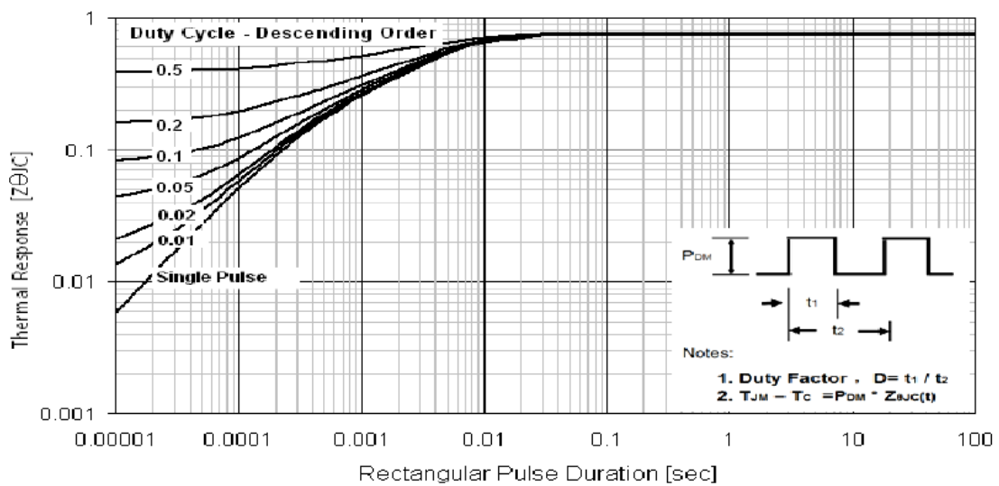
Transient Thermal Response Curve For JCS4N65REI/VEI
