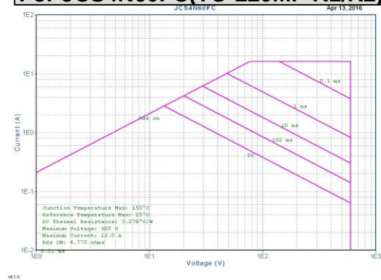
Maximum Safe Operating Area For JCS4N60FC(TO-220MF-K1/K2)
