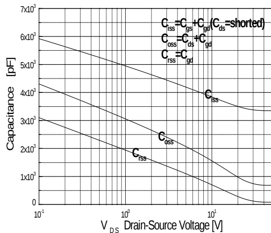
Capacitance Characteristics
