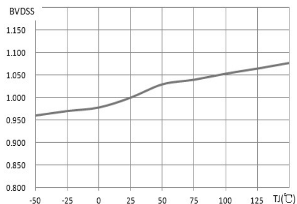
Normalized BVdss vs. temperature
