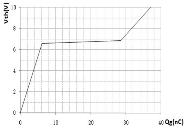
Gate charge vs. Vgs
