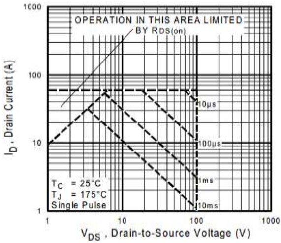
Maximum Safe Operating Area (JCS3910V/R/C/S)
