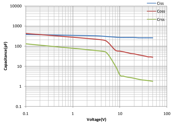
Capacitance Characteristics
