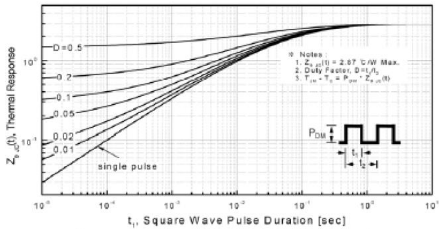
Transient Thermal Response Curve For JCS2N65CB
