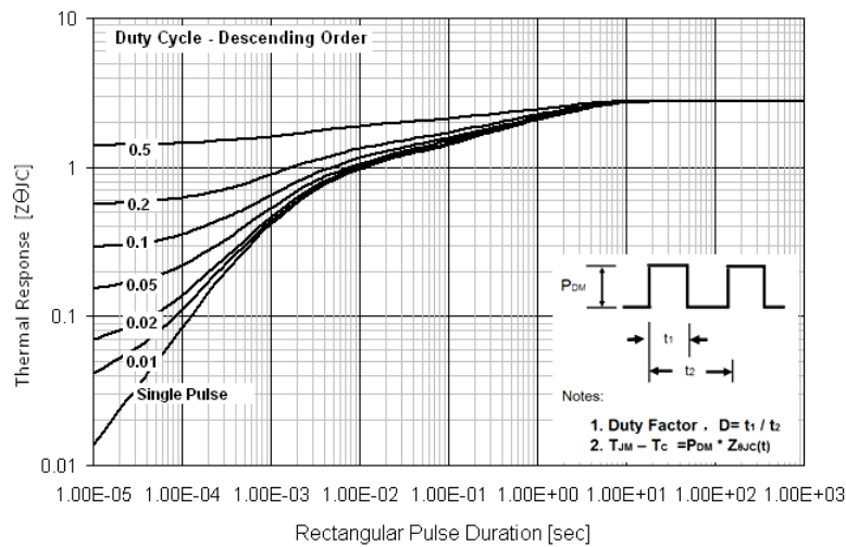
Transient Thermal Response Curve For JCS2N65FB
