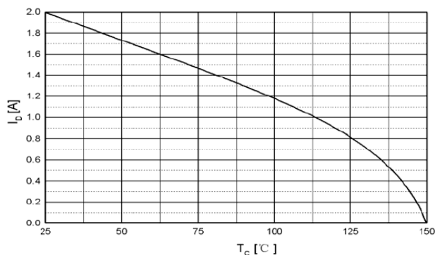
Maximum Drain Current vs. Case Temperature
