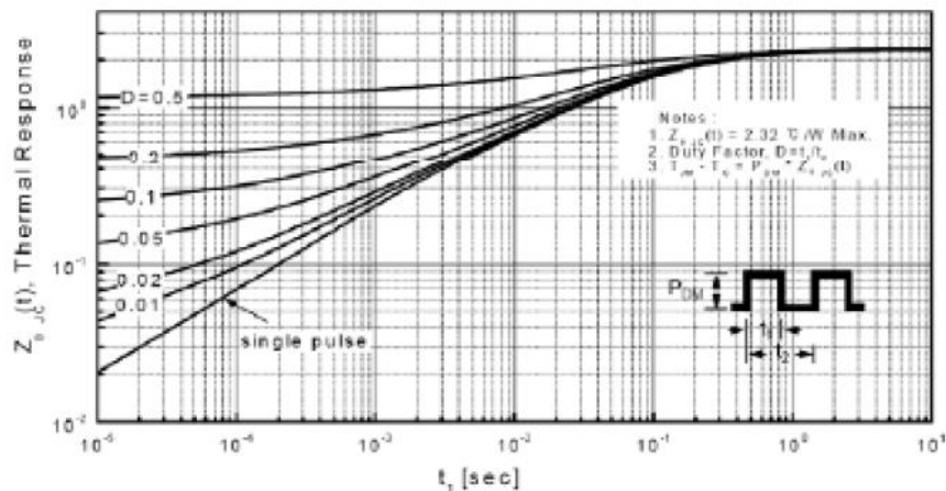
Transient Thermal Response Curve For JCS2N65FB
