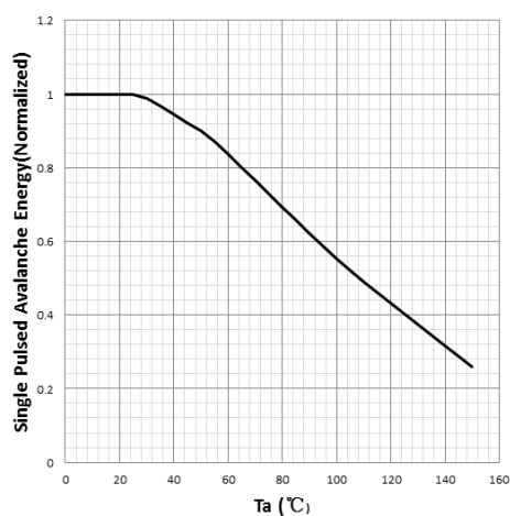
Avalanche Energy vs. Temperature
