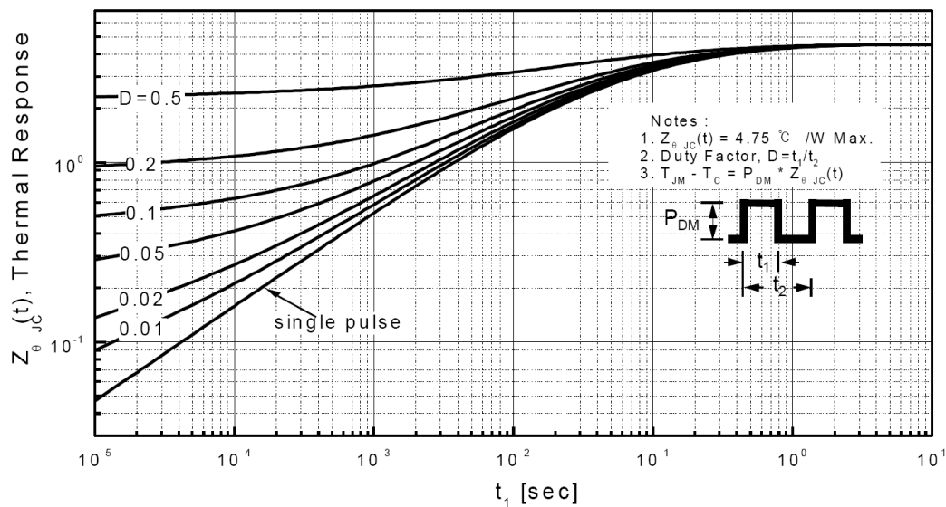
Transient Thermal Response Curve For JCS1SN65VC/RC
