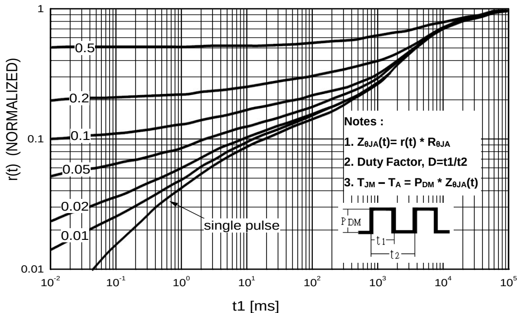
Transient Thermal Response Curve For JCS1SN65TC
