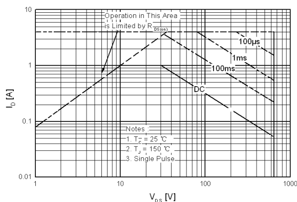
Maximum Safe Operating Area For JCS1SN65VC/RC
