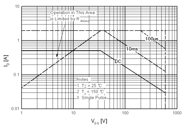
Maximum Safe Operating Area For JCS1HN65TC
