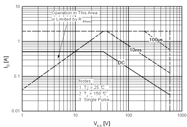
Maximum Safe Operating Area For JCS1HN65T
