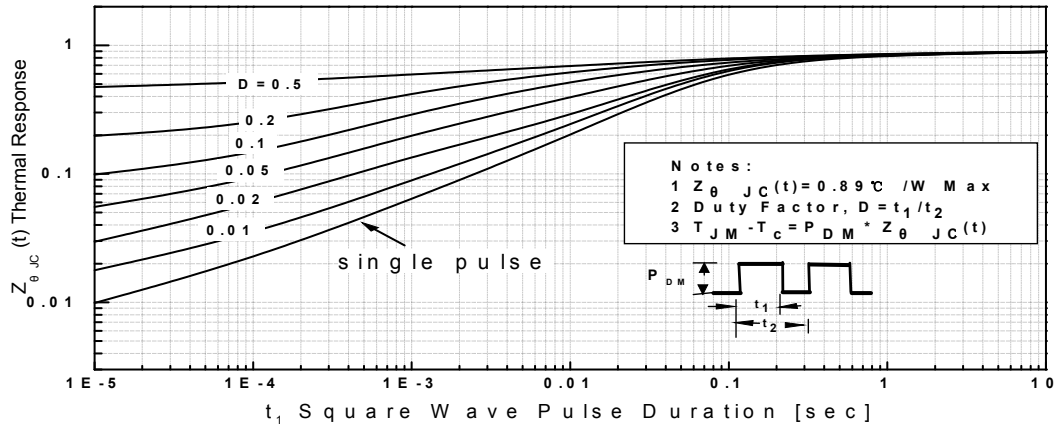
Transient Thermal Response Curve For JCS19N20F
