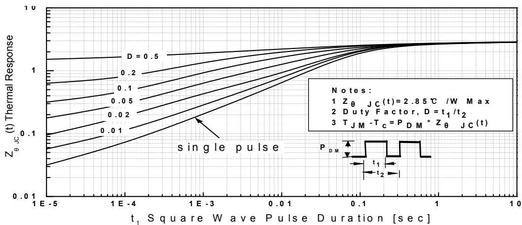
Transient Thermal Response Curve For JCS19N20F
