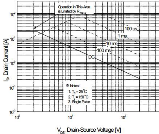
Maximum Safe Operating Area For JCS19N20F
