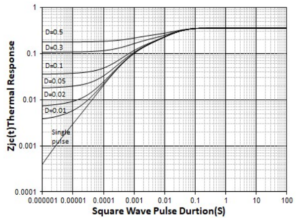
Transient Thermal Response Curve For JCS170N08I(TO-220C)
