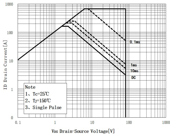
Maximum Safe Operating Area For JCS170N08I(TO-220C)
