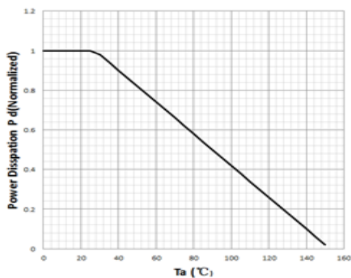
Power Dissipation vs. Temperature
