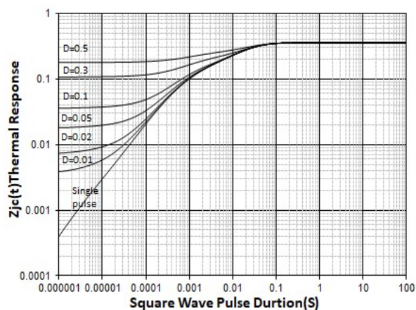
Transient Thermal Response Curve For JCS150N10I(TO-220C)
