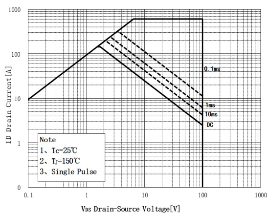
Maximum Safe Operating Area For JCS150N10I(TO-220C)
