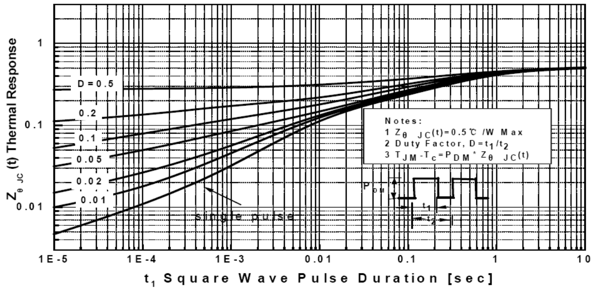
Transient Thermal Response Curve For JCS12N60BC/CC/SC
