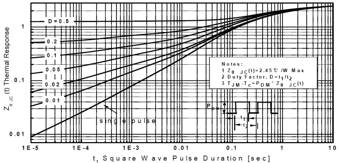
Transient Thermal Response Curve For JCS12N60FC
