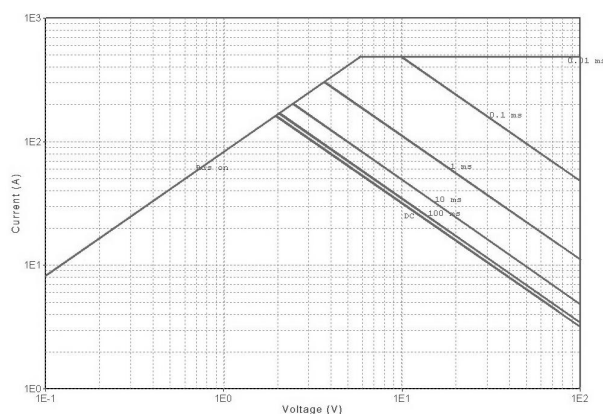
Maximum Safe Operating Area For JCS120N10I(TO-220C)
