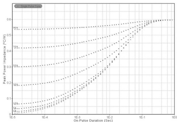
Transient Thermal Response Curve For JCS120N10I(TO-220C)
