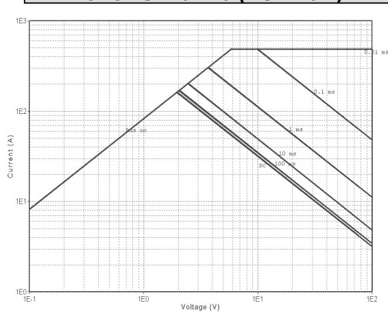
Maximum Safe Operating Area For JCS120N10I(TO-220C)
