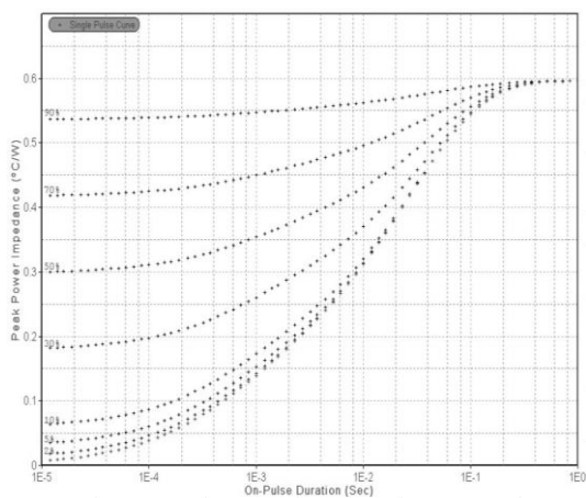
Transient Thermal Response Curve For JCS120N08I
