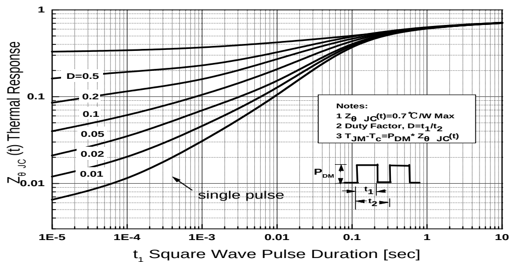
Transient Thermal Response Curve For JCS10N65CC/BC/SC
