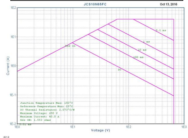
Maximum Safe Operating Area For JCS10N65FC
