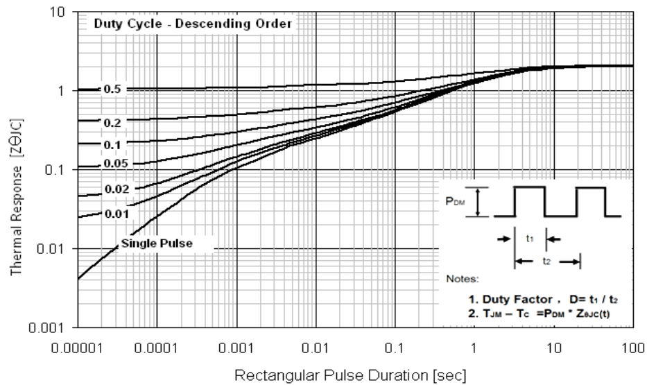
Transient Thermal Response Curve For JCS10N65FC
