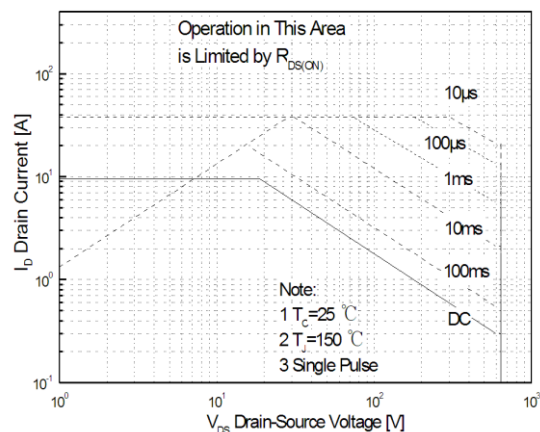
Maximum Safe Operating Area For JCS10N65CC/BC/SC
