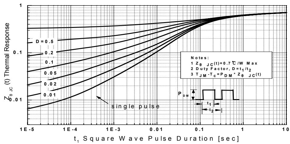
Transient Thermal Response Curve For JCS10N60BT
