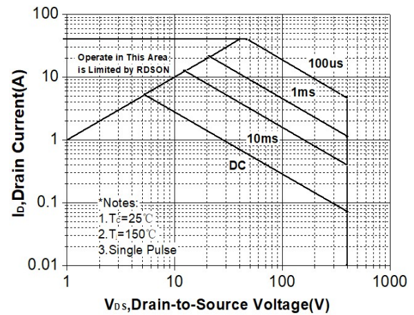
Maximum Safe Operating Area For JCS10AN40FC
