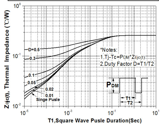
Fig.4 Transient Thermal Response Curve
