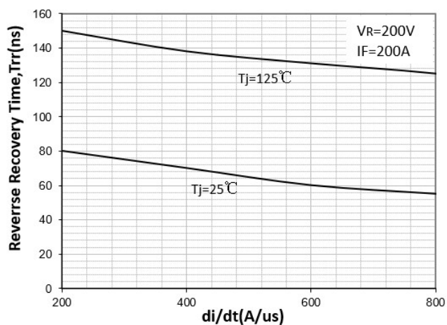
Fig.3 Reverse recovery time versus dI_F/dt
