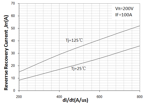
Fig.4 Peak reverse recovery current versus di/dt
