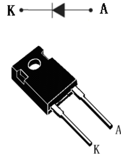
TO-247-2L
