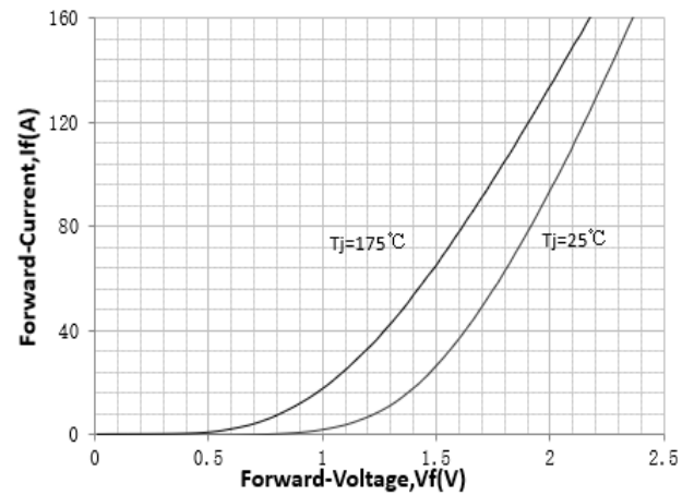
Diode Characteristic
