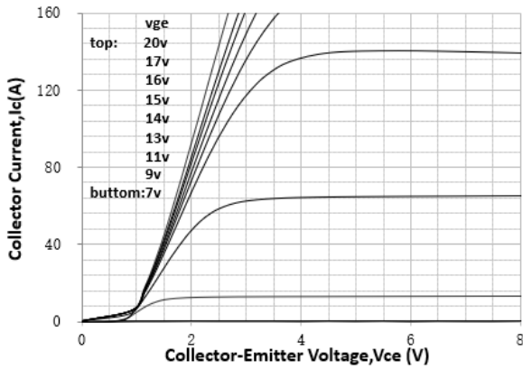
Output Characteristics (25°C)
