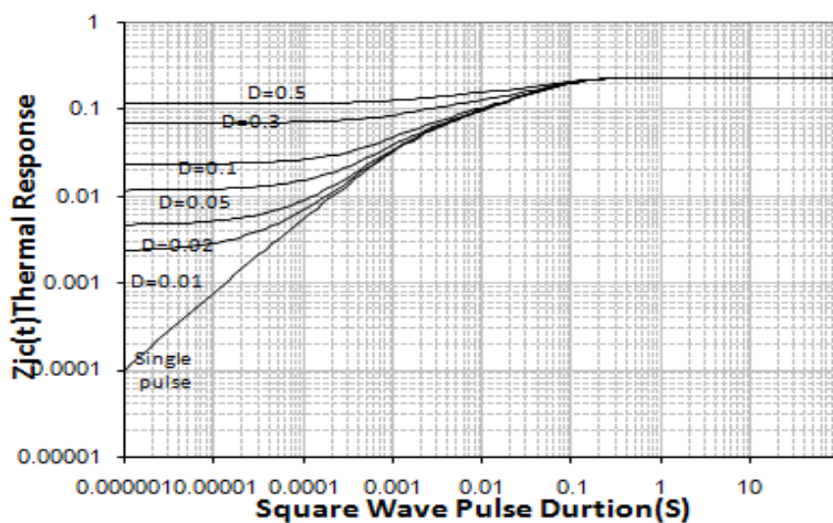
Transient Thermal Response Curve
