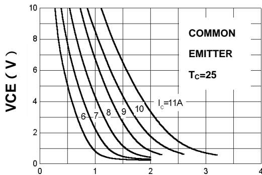
VCE - IB
