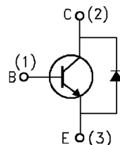
TO-220C-S1
